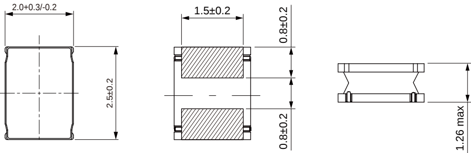
Dimensions: [mm]
